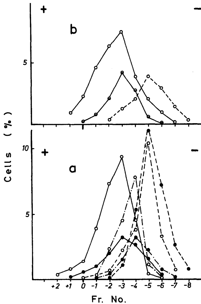
Fig. 1: Electrophoretic Distribution Profiles of Granulopoiesis. a) —●— promyelocytes and myelocytes -.- metamyelocytes and rods --- segments ● normal, ○ chronic myeloid leukemia b) ●—● myeloblasts ○—○ promyelocytes and myelocytes ○--○ segments
